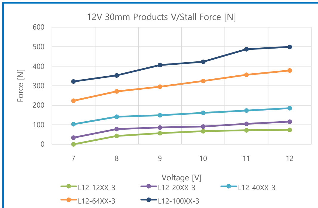
Figure2-2 . Voltage /Stall Force[N] (12V / 27mmProducts)
