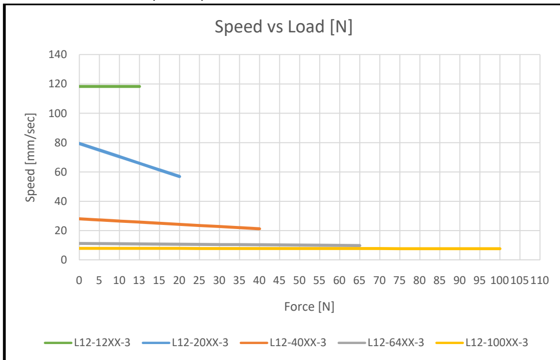
Figure1-2 . SPEED VS LOAD (12 VDC)
