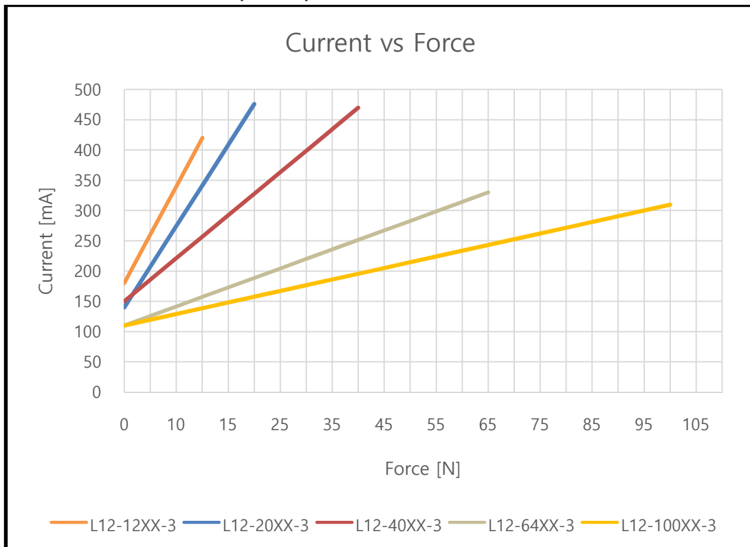
Figure1-1 . CURRENT VS FORCE (12 VDC)
